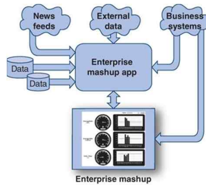
FIGURE 6.17 Architecture of enterprise mashup application
