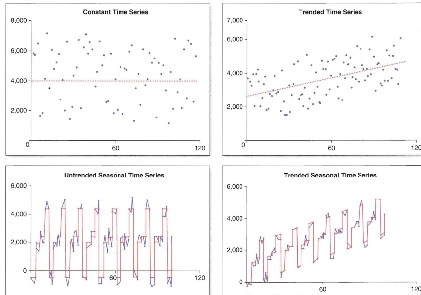
FIGURE 6.21 Example of time-series regression models
