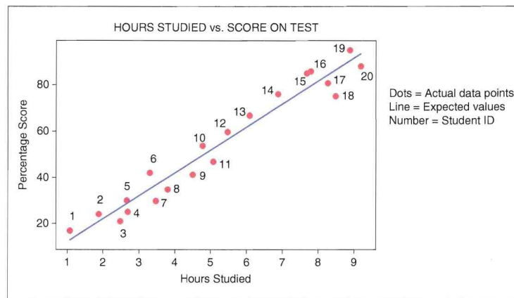
FIGURE 6.20 Simple linear regression model
